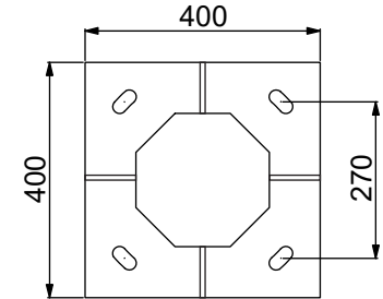
BASE PLATE # 16mm x 400 x 400
